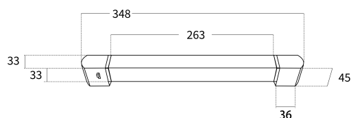
4863-1U (mm)
